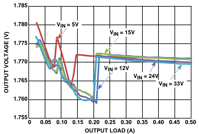
FIGURE 16. V OUT REGULATION vs LOAD, PFM, V OUT = 1.8V
