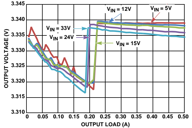
FIGURE 14. V OUT REGULATION vs LOAD, PFM, V OUT = 3.3V
