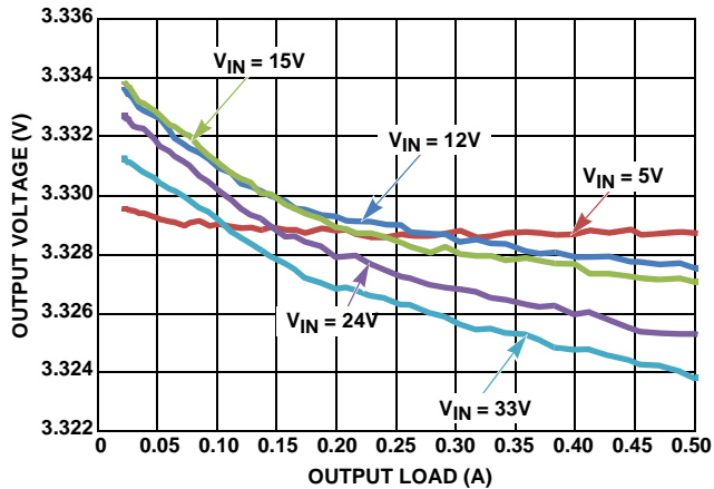
FIGURE 13. V OUT REGULATION vs LOAD, PWM, V OUT = 3.3V
