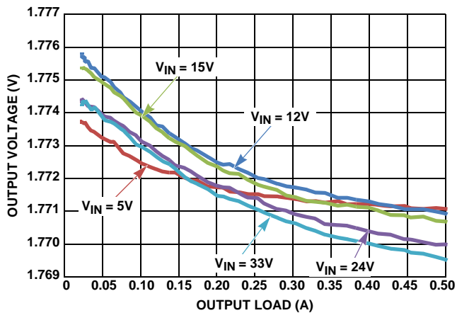
FIGURE 15. V OUT REGULATION vs LOAD, PWM, V OUT = 1.8V
